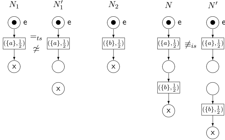
Figure 4. The equivalences between \equiv_{is} and =_{ts} are not congruences
