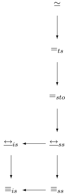
Figure 2. Interrelations of the stochastic equivalences
