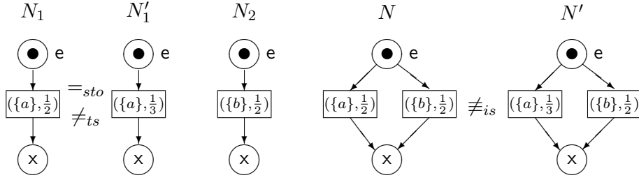
Figure 3. The equivalences between \equiv_{is} and =_{sto} are not congruences
