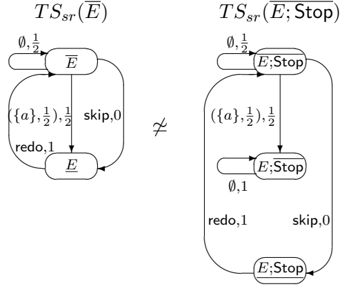
Figure 5. The sr -transition systems of \overline{E} and \overline{E; \text{Stop}} for E = (\{a\}, \frac{1}{2})
