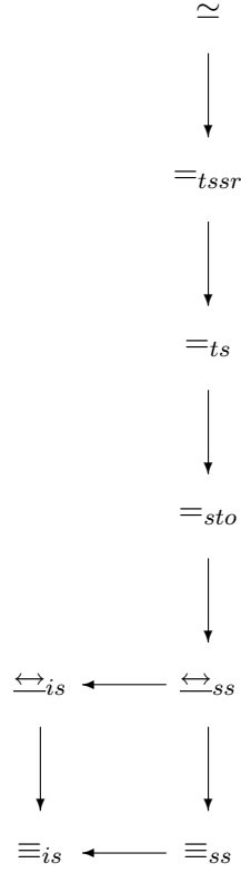
Figure 6. Interrelations of the stochastic equivalences and the new congruence
