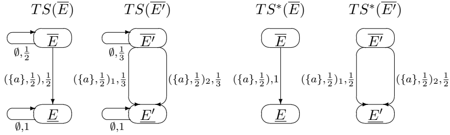
Figure 1. A problem with the stochastic isomorphism based on transition systems with empty loops
